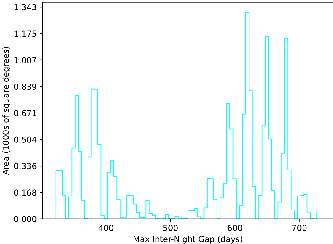
roll_pause_mjdp270_v3.4_10yrs WFD u band: Max Inter-Night Gap
