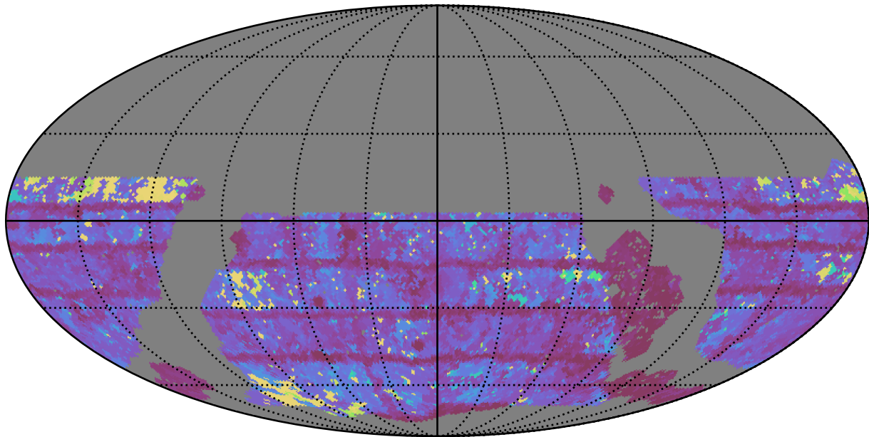
roll_pause_mjdp270_v3.4_10yrs WFD i band: Max Inter-Night Gap
