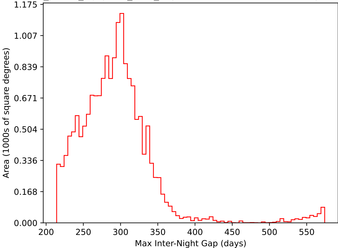
roll_pause_mjdp270_v3.4_10yrs WFD i band: Max Inter-Night Gap
