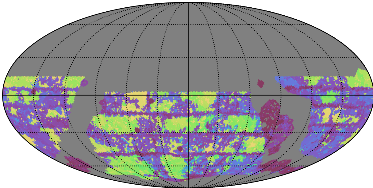
roll_pause_mjdp270_v3.4_10yrs WFD g band: Max Inter-Night Gap
