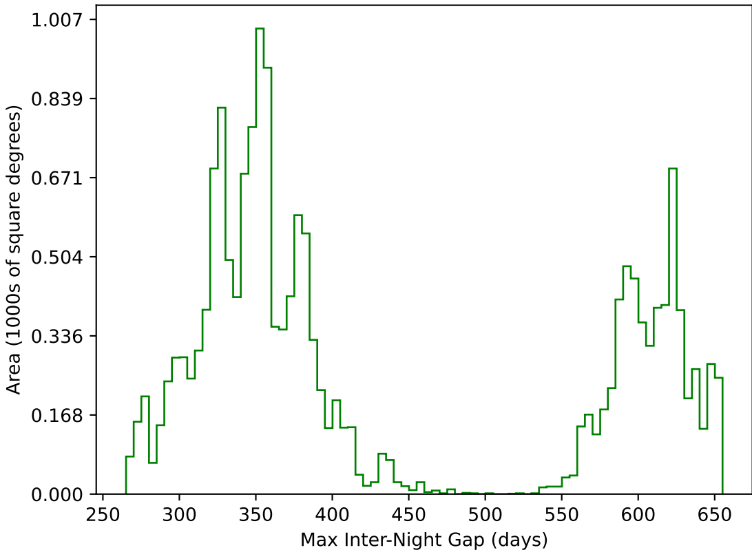
roll_pause_mjdp270_v3.4_10yrs WFD g band: Max Inter-Night Gap
