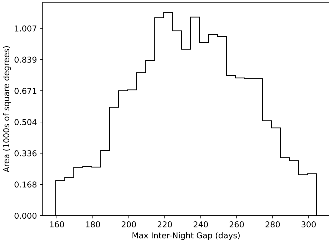
roll_pause_mjdp270_v3.4_10yrs WFD all bands: Max Inter-Night Gap
