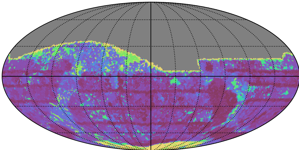
roll_pause_mjdp270_v3.4_10yrs All sky z band: Max Inter-Night Gap
