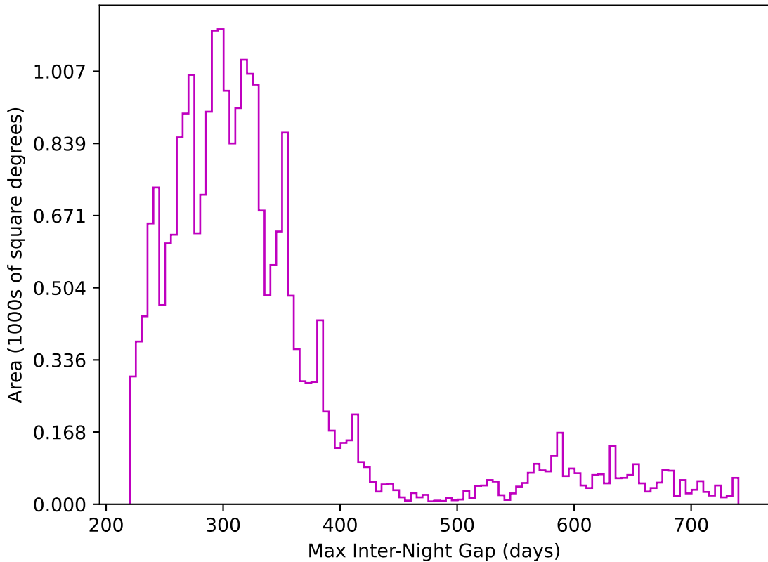
roll_pause_mjdp270_v3.4_10yrs All sky z band: Max Inter-Night Gap
