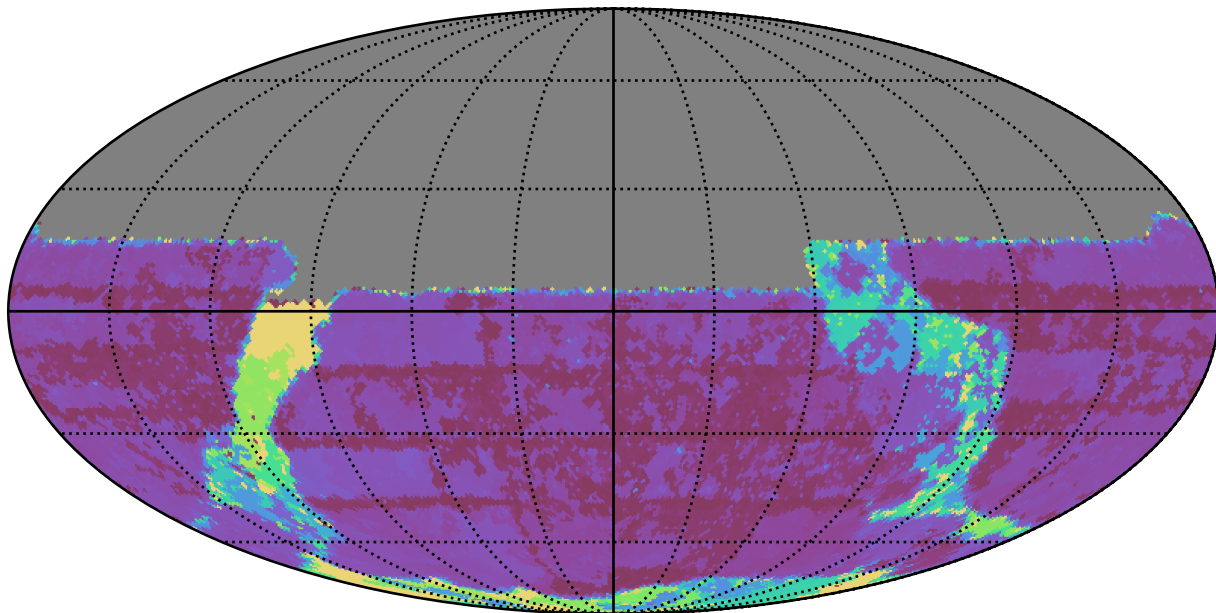
roll_pause_mjdp270_v3.4_10yrs All sky u band: Max Inter-Night Gap
