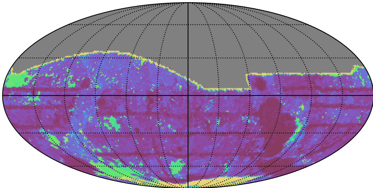
roll_pause_mjdp270_v3.4_10yrs All sky r band: Max Inter-Night Gap
