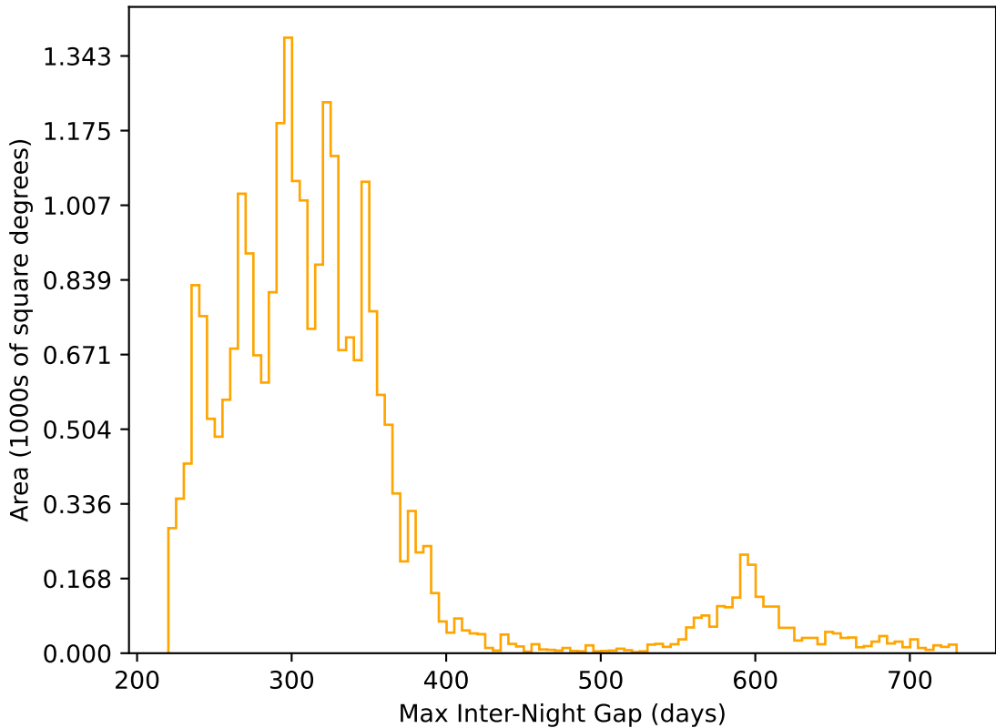
roll_pause_mjdp270_v3.4_10yrs All sky r band: Max Inter-Night Gap
