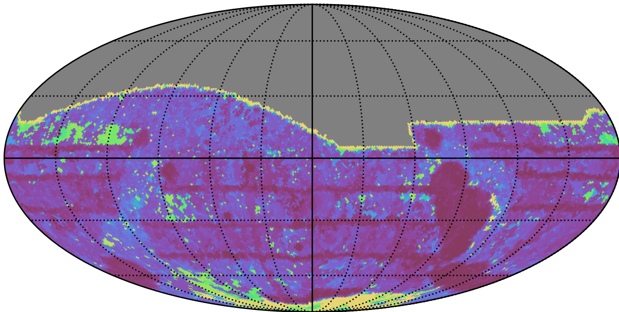
roll_pause_mjdp270_v3.4_10yrs All sky i band: Max Inter-Night Gap
