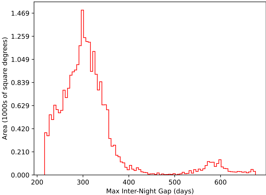
roll_pause_mjdp270_v3.4_10yrs All sky i band: Max Inter-Night Gap
