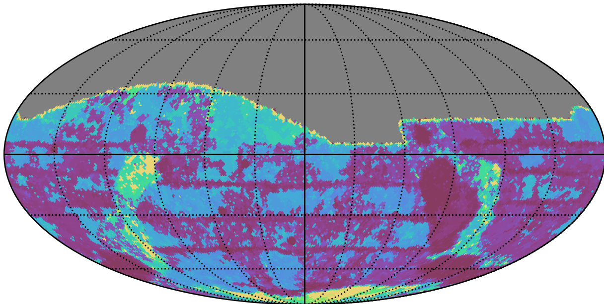
roll_pause_mjdp270_v3.4_10yrs All sky g band: Max Inter-Night Gap
