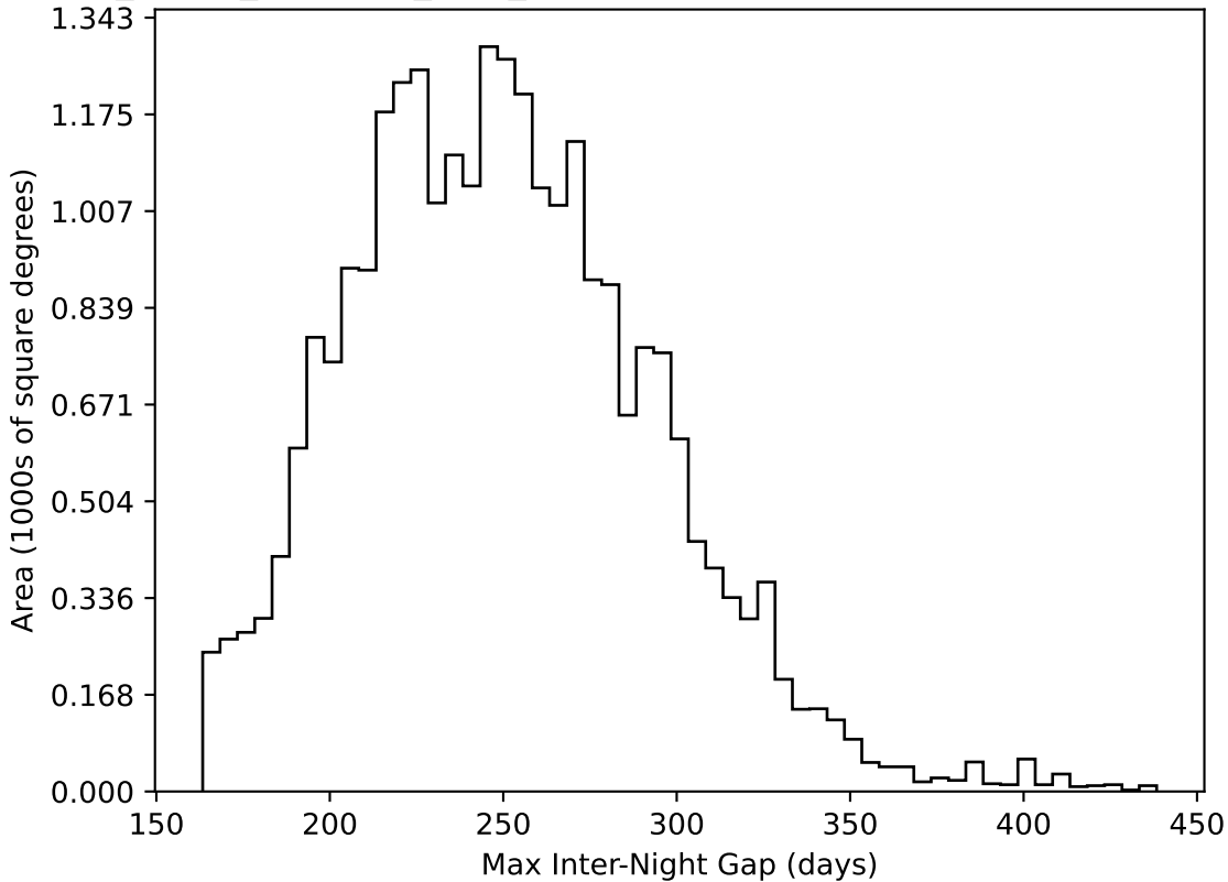
roll_pause_mjdp270_v3.4_10yrs All sky all bands: Max Inter-Night Gap
