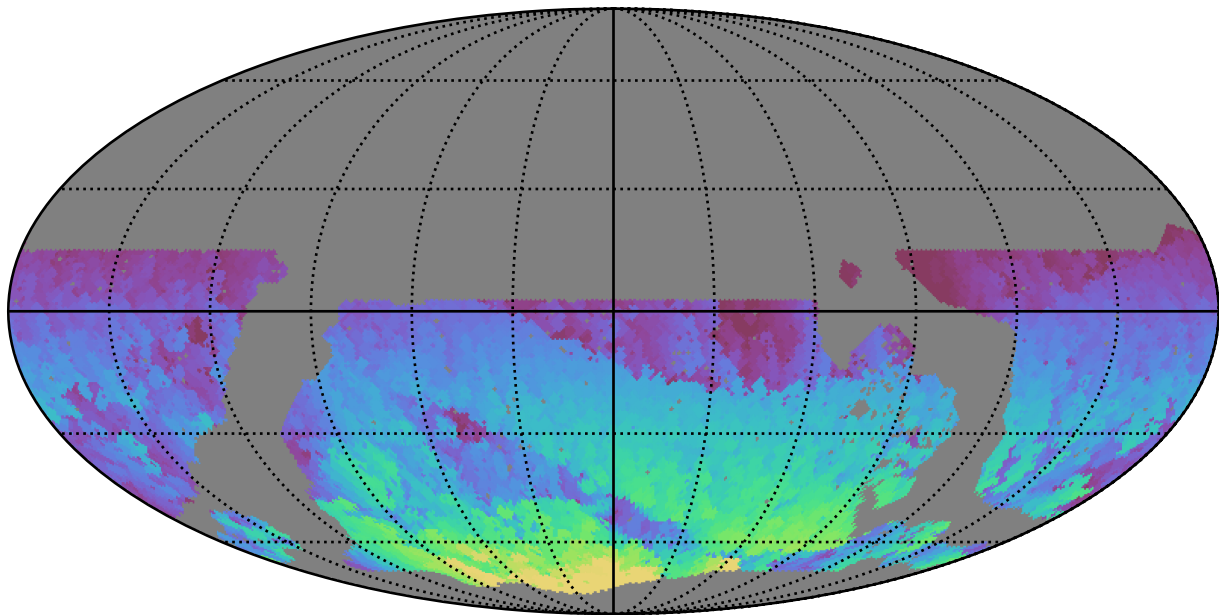
roll_pause_mjdp270_v3.4_10yrs WFD z band: Max HA
