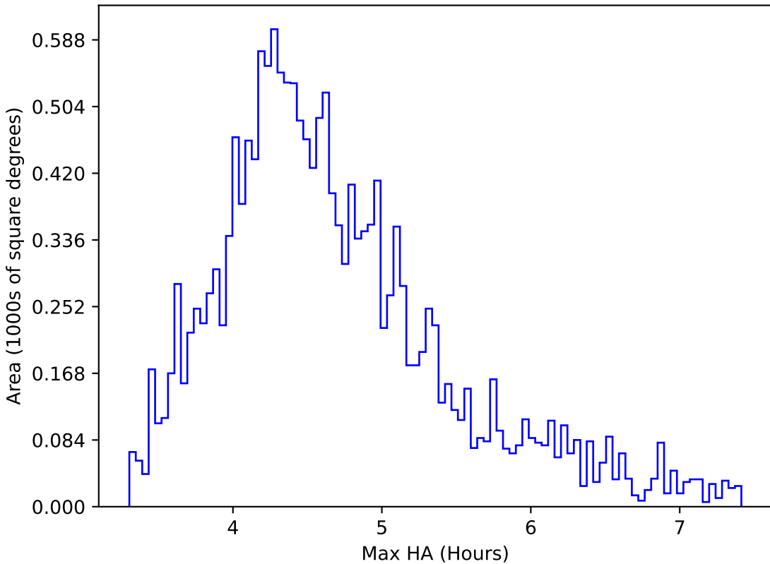
roll_pause_mjdp270_v3.4_10yrs WFD y band: Max HA
