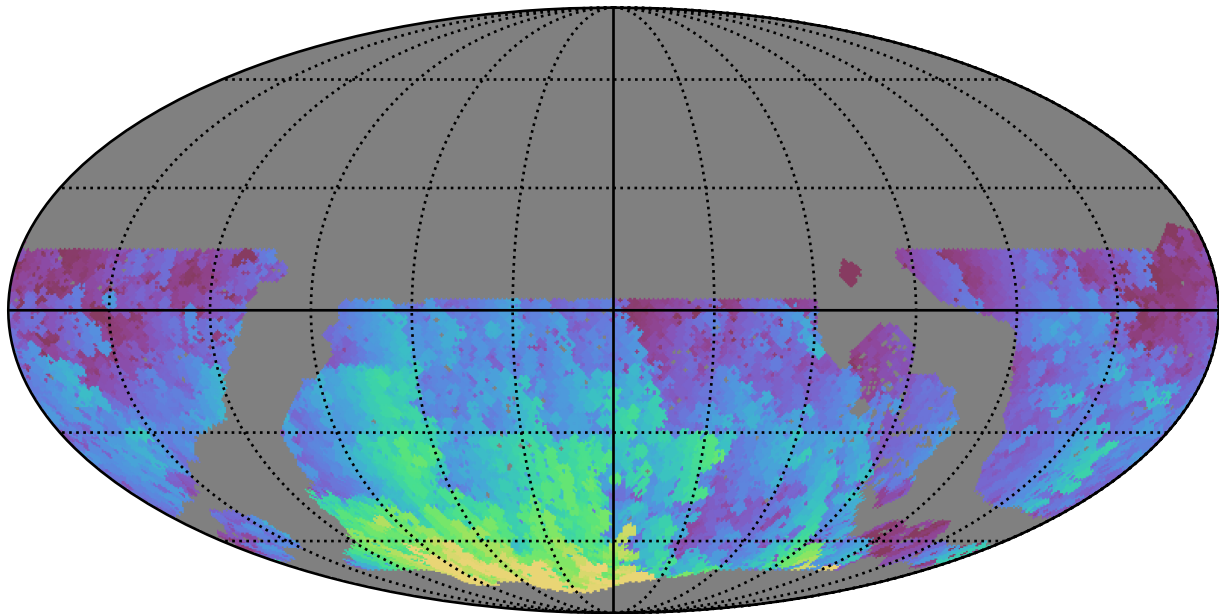
roll_pause_mjdp270_v3.4_10yrs WFD u band: Max HA
