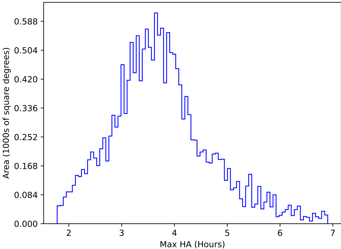
roll_pause_mjdp270_v3.4_10yrs WFD u band: Max HA
