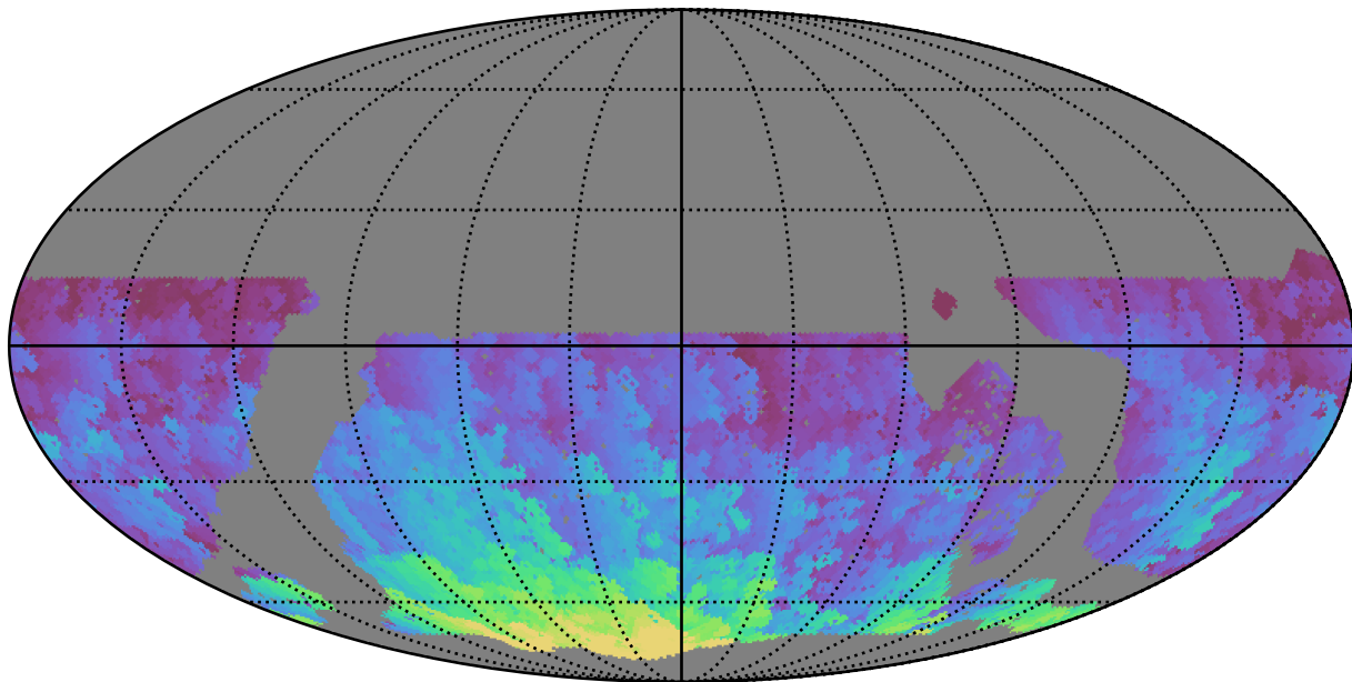
roll_pause_mjdp270_v3.4_10yrs WFD r band: Max HA
