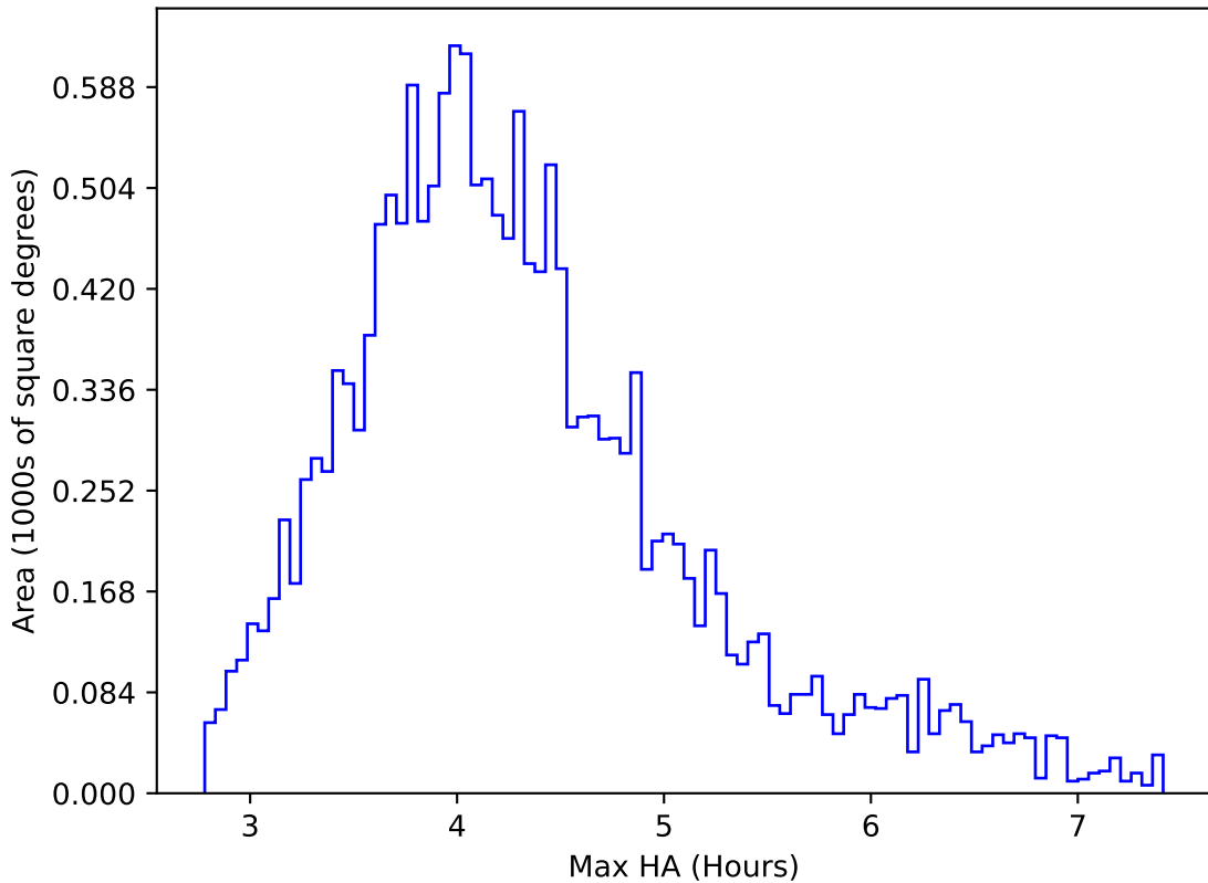
roll_pause_mjdp270_v3.4_10yrs WFD r band: Max HA
