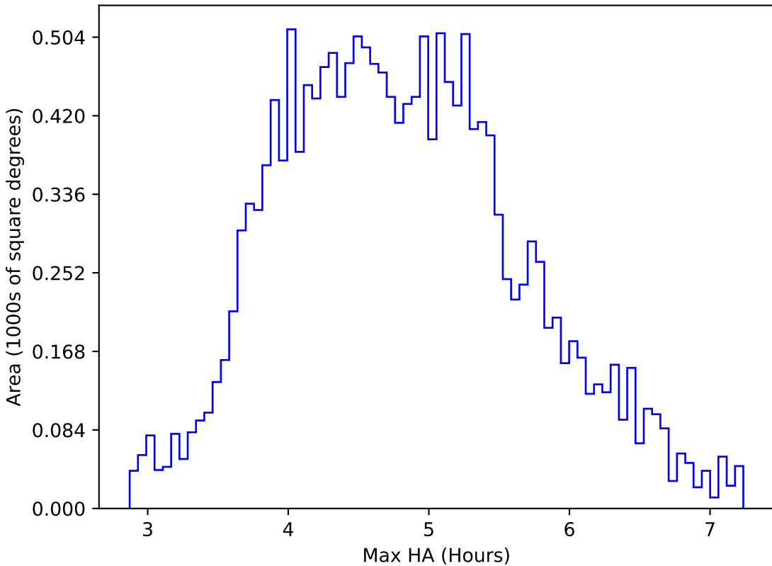
roll_pause_mjdp270_v3.4_10yrs WFD i band: Max HA
