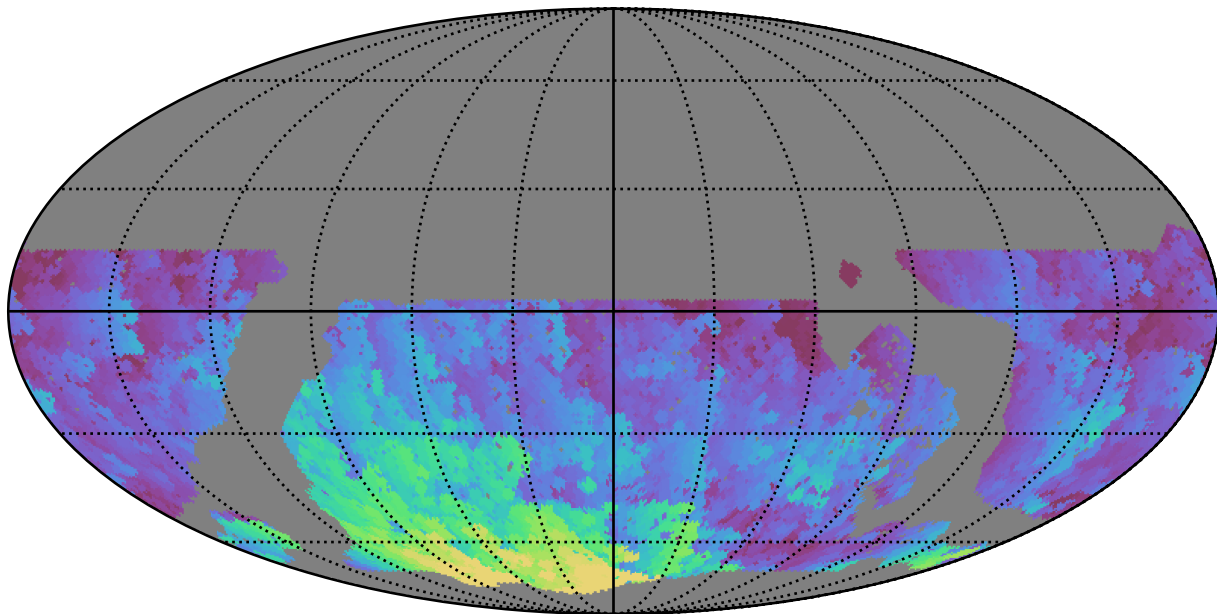
roll_pause_mjdp270_v3.4_10yrs WFD g band: Max HA
