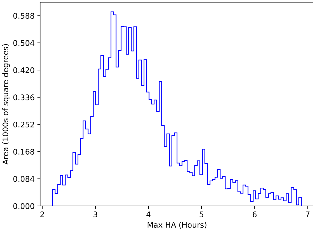
roll_pause_mjdp270_v3.4_10yrs WFD g band: Max HA
