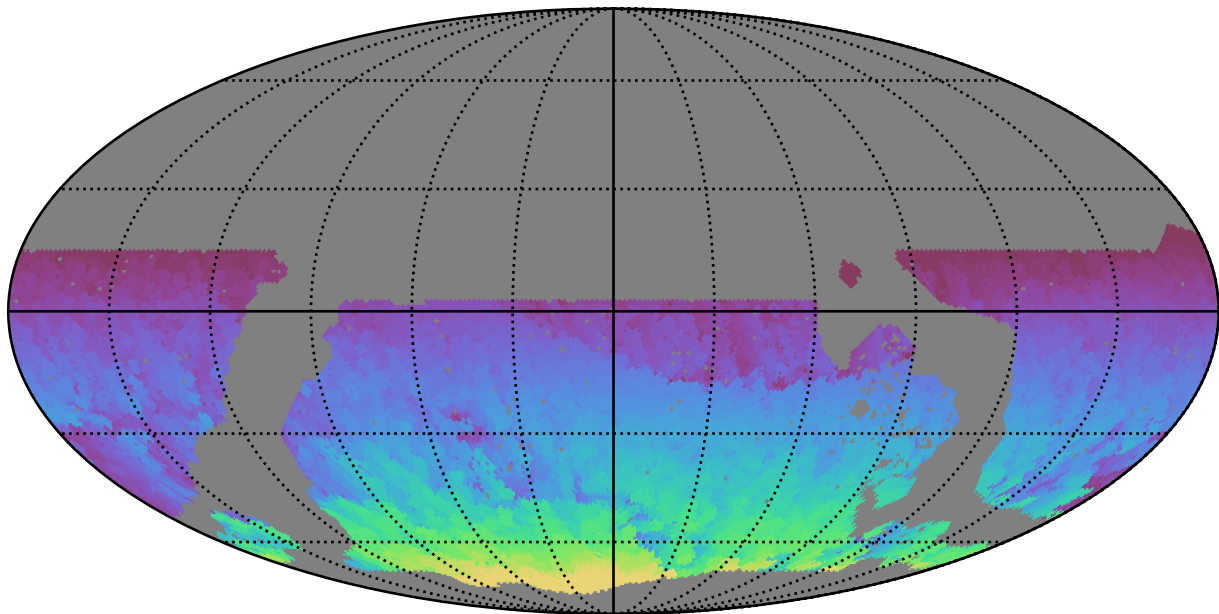
roll_pause_mjdp270_v3.4_10yrs WFD all bands: Max HA
