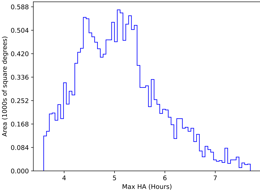
roll_pause_mjdp270_v3.4_10yrs WFD all bands: Max HA
