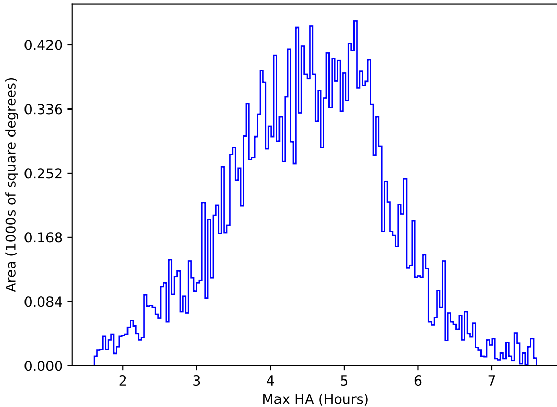
roll_pause_mjdp270_v3.4_10yrs All sky z band: Max HA
