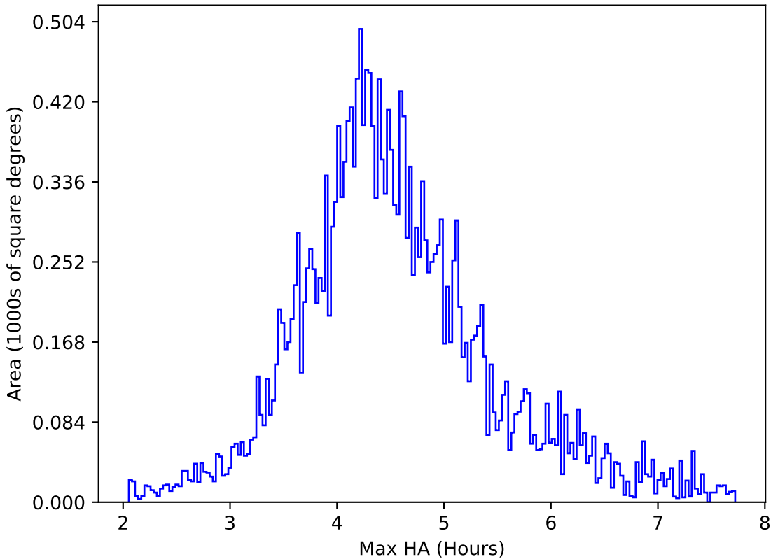
roll_pause_mjdp270_v3.4_10yrs All sky y band: Max HA
