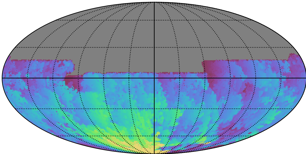
roll_pause_mjdp270_v3.4_10yrs All sky u band: Max HA
