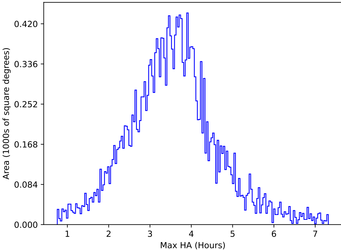
roll_pause_mjdp270_v3.4_10yrs All sky u band: Max HA
