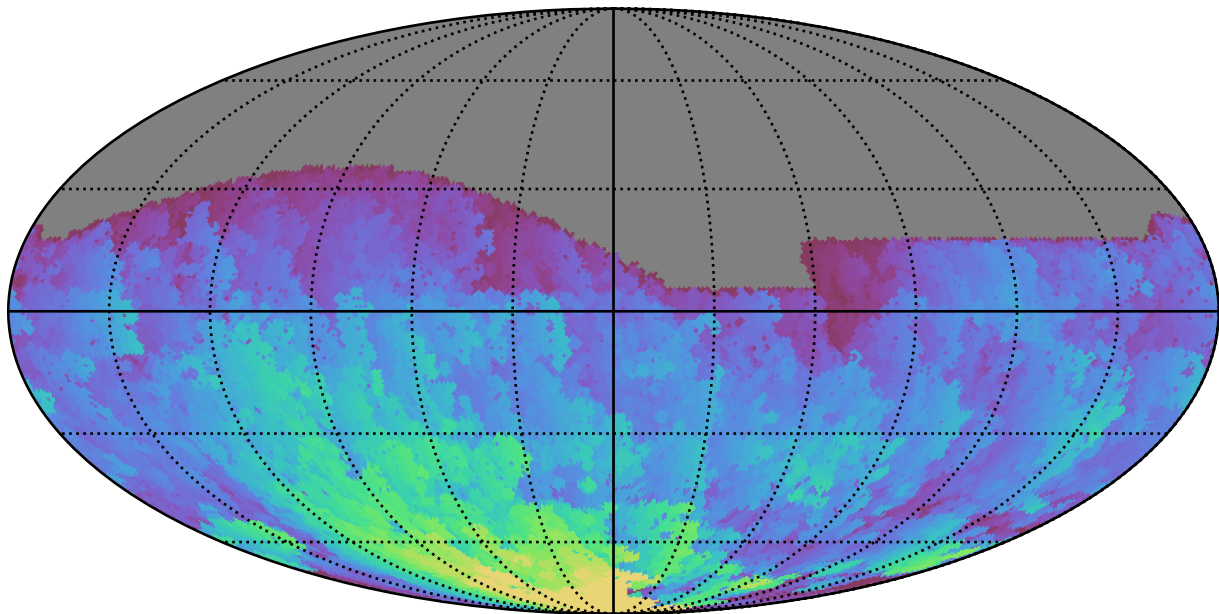
roll_pause_mjdp270_v3.4_10yrs All sky g band: Max HA
