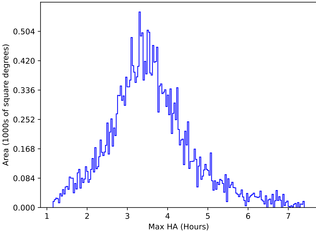
roll_pause_mjdp270_v3.4_10yrs All sky g band: Max HA
