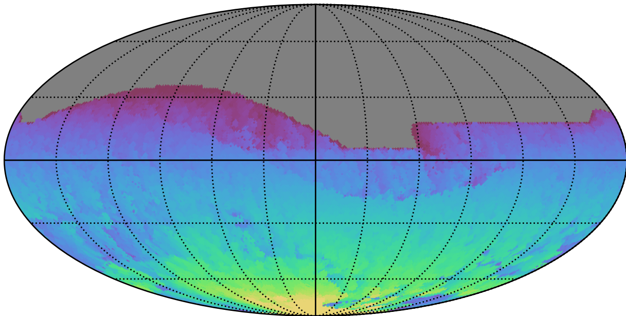
roll_pause_mjdp270_v3.4_10yrs All sky all bands: Max HA
