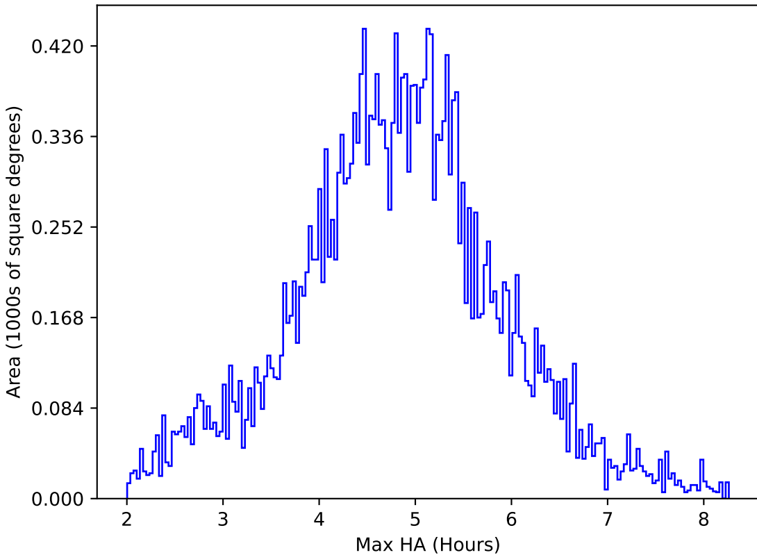
roll_pause_mjdp270_v3.4_10yrs All sky all bands: Max HA
