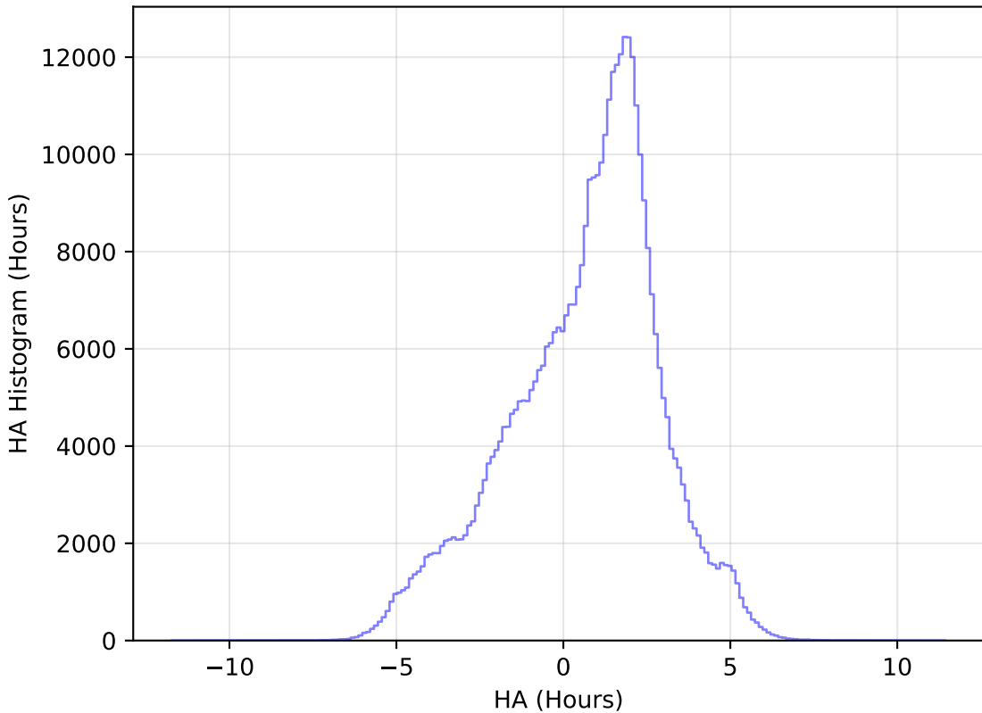
roll_pause_mjdp270_v3.4_10yrs WFD z band: HA Histogram
