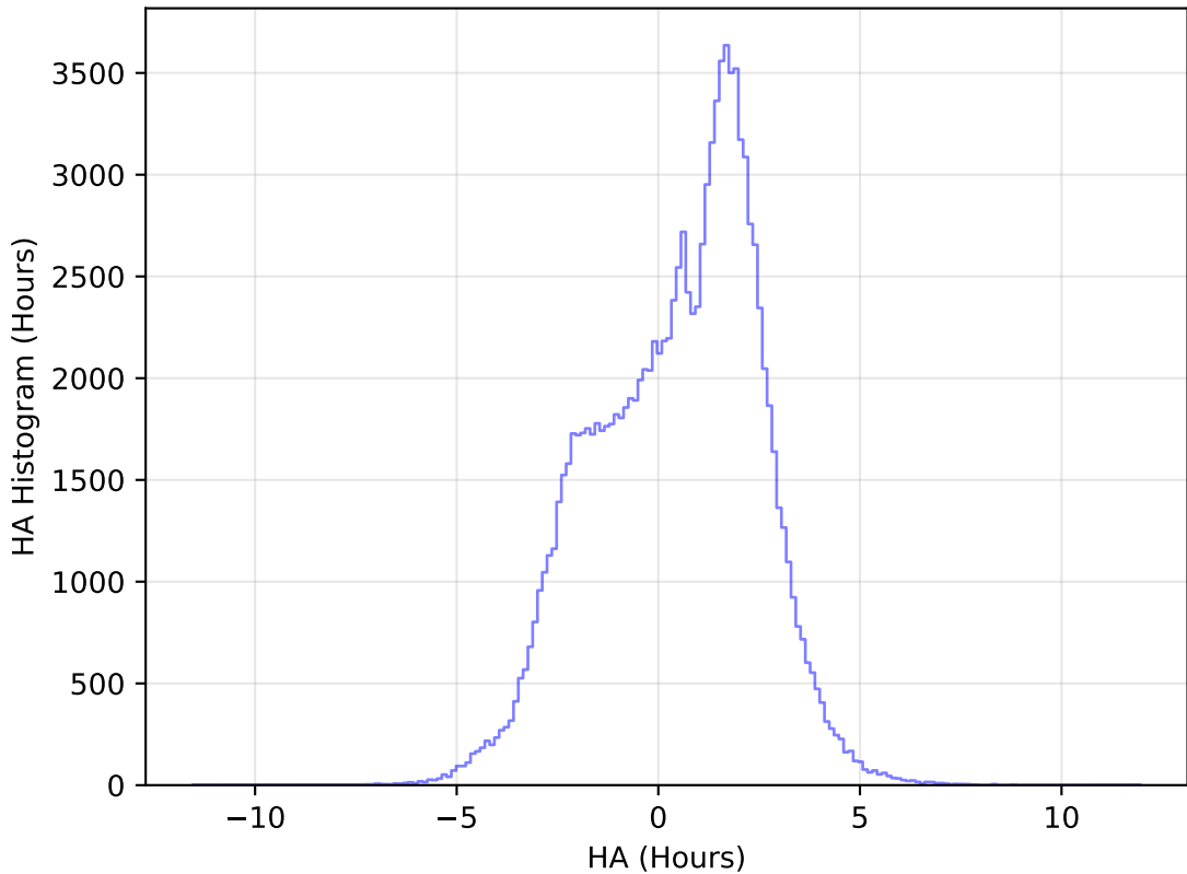
roll_pause_mjdp270_v3.4_10yrs WFD u band: HA Histogram
