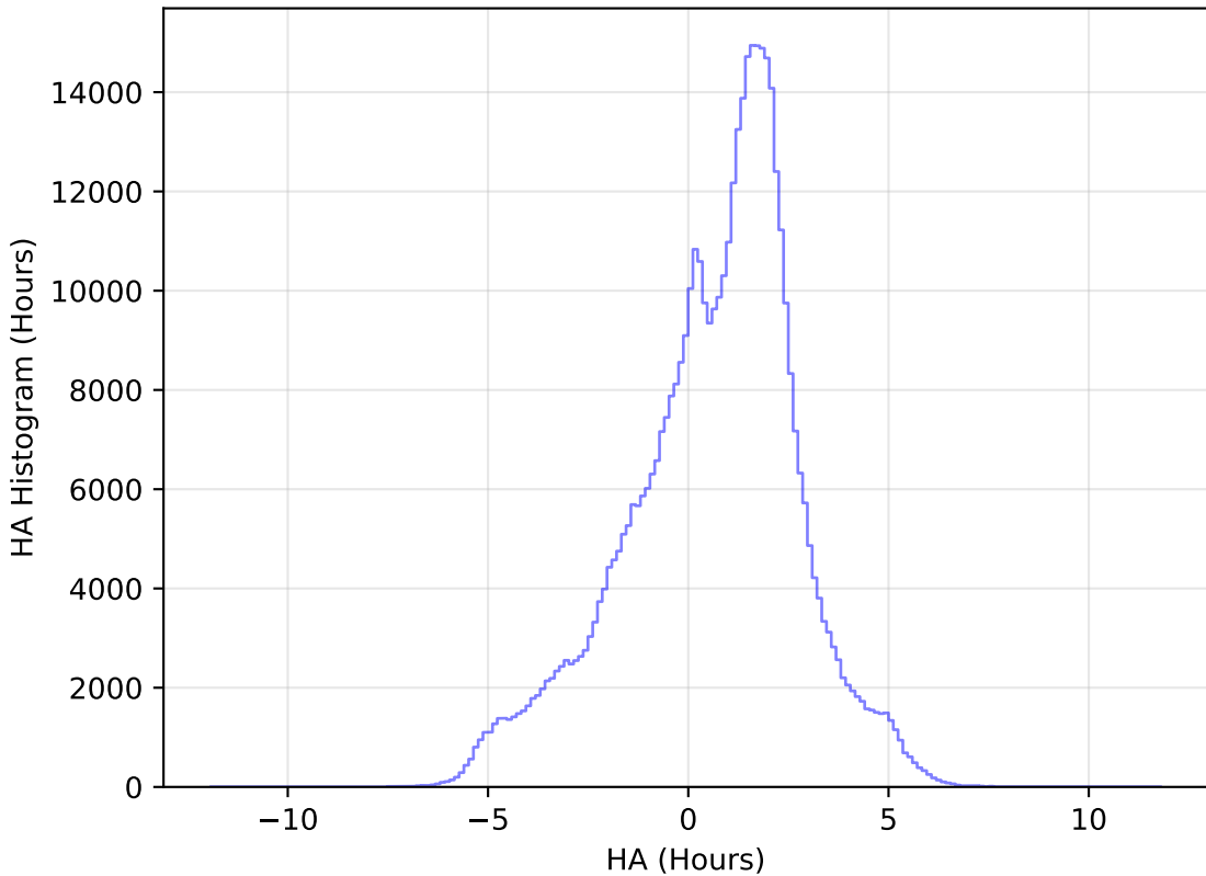
roll_pause_mjdp270_v3.4_10yrs WFD i band: HA Histogram
