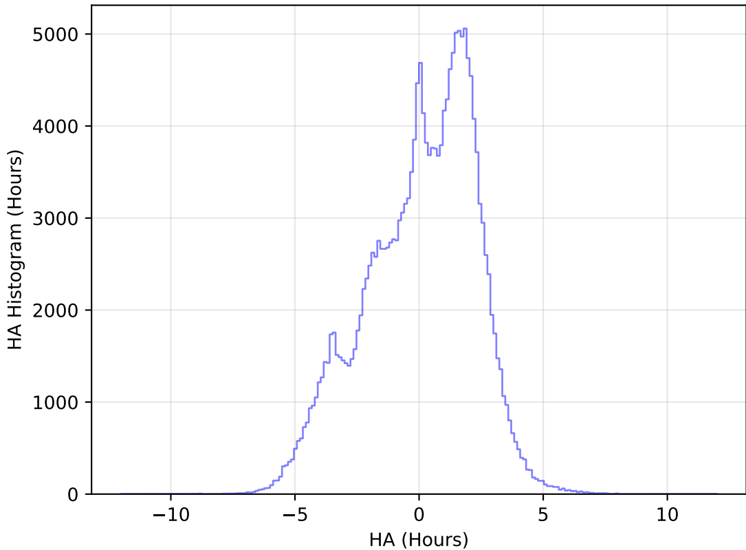
roll_pause_mjdp270_v3.4_10yrs WFD g band: HA Histogram
