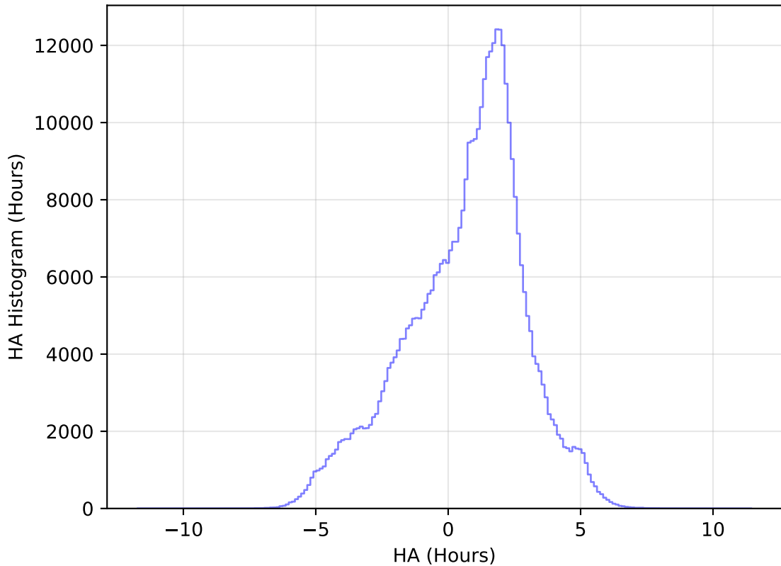
roll_pause_mjdp270_v3.4_10yrs All sky z band: HA Histogram
