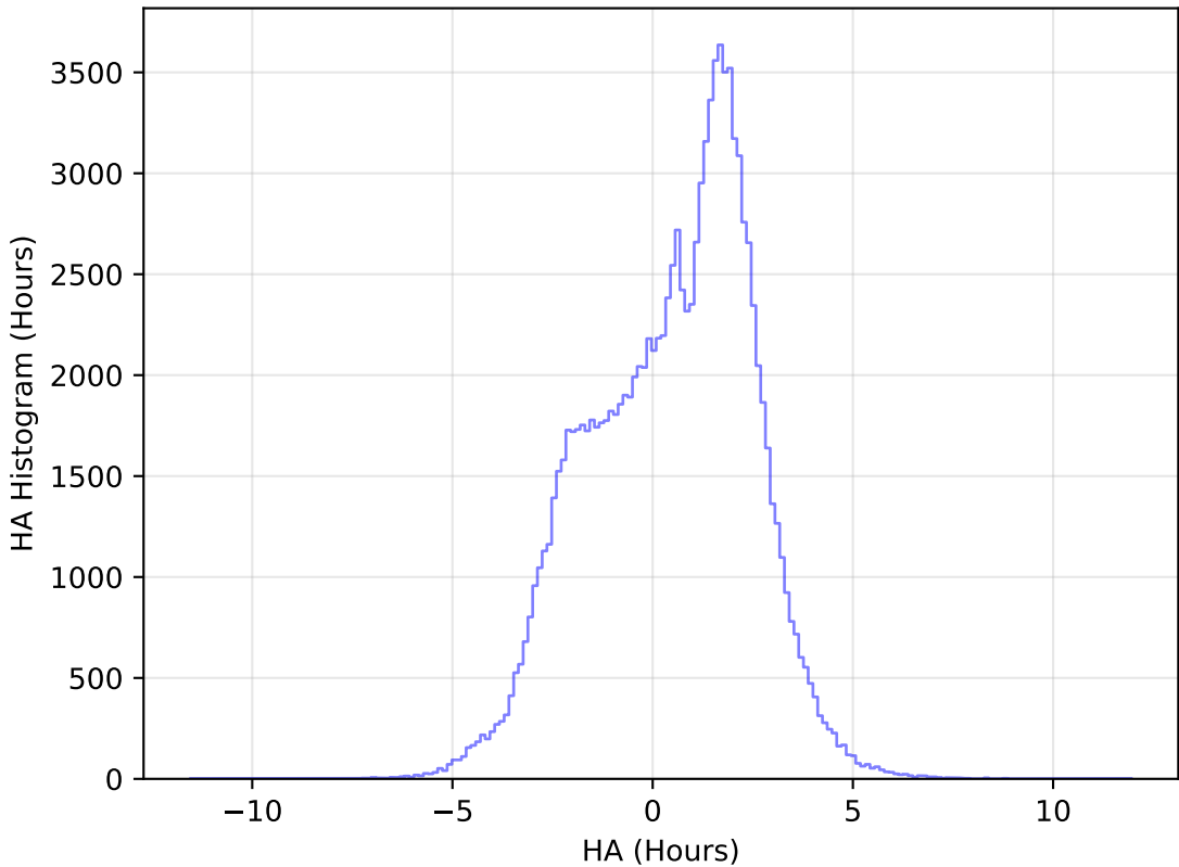
roll_pause_mjdp270_v3.4_10yrs All sky u band: HA Histogram
