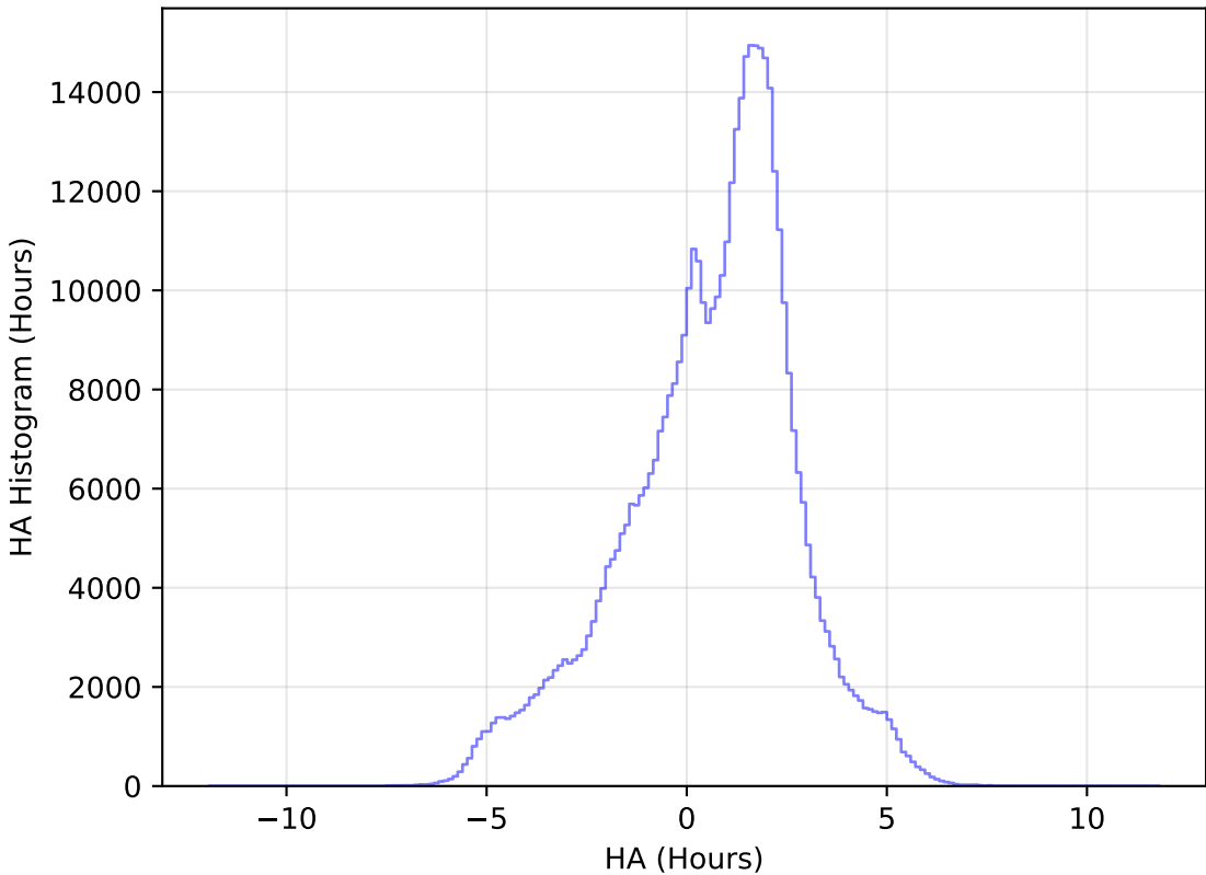
roll_pause_mjdp270_v3.4_10yrs All sky i band: HA Histogram
