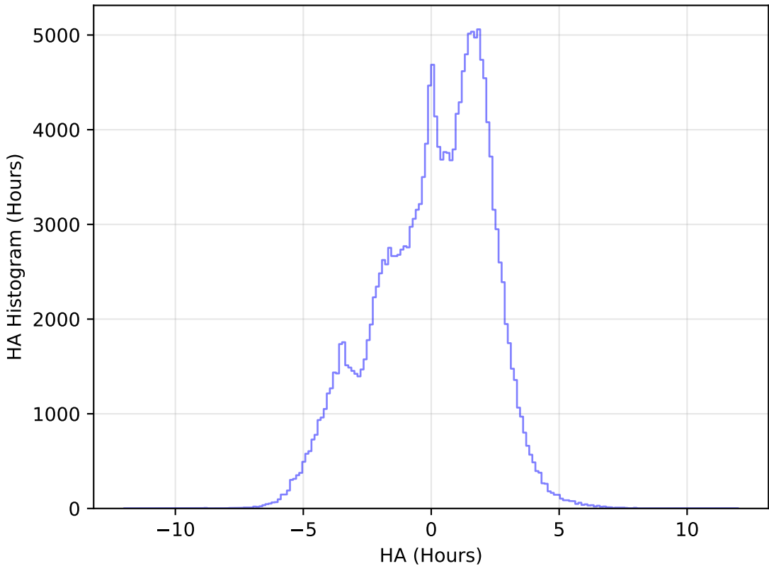
roll_pause_mjdp270_v3.4_10yrs All sky g band: HA Histogram
