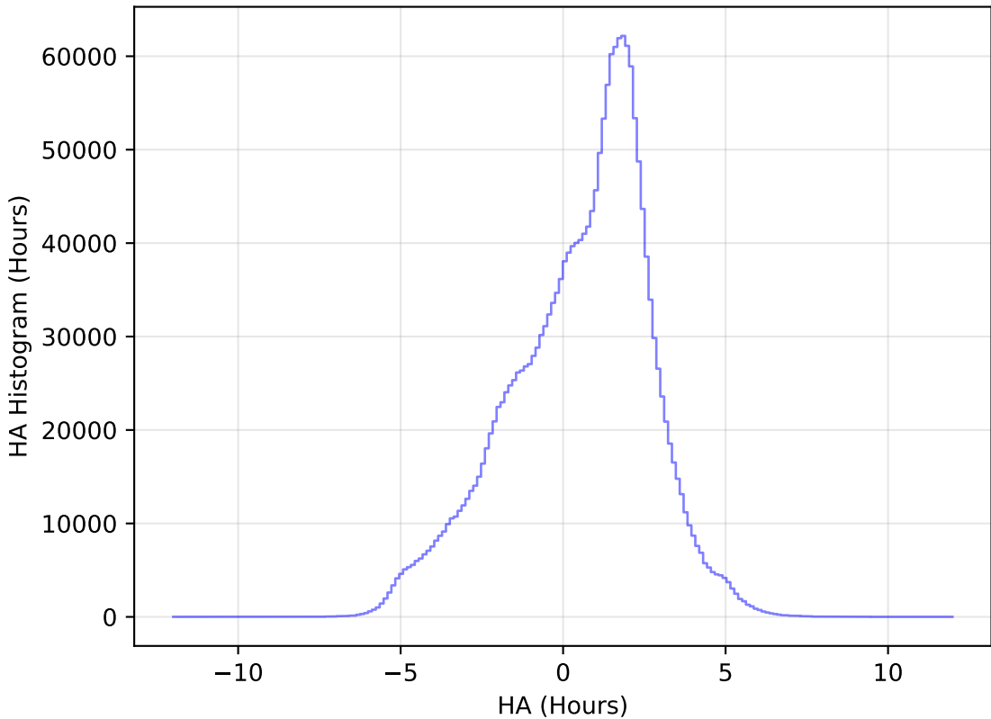
roll_pause_mjdp270_v3.4_10yrs All sky all bands: HA Histogram
