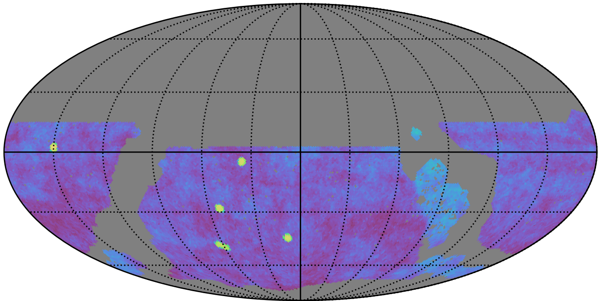
roll_pause_mjdp270_v3.4_10yrs gri WFD: Fraction of visits in pairs (10-60 min)
