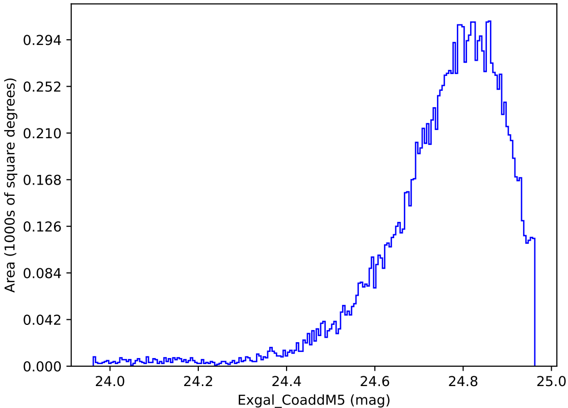
roll_pause_mjdp270_v3.4_10yrs WFD y band: Exgal_CoaddM5
