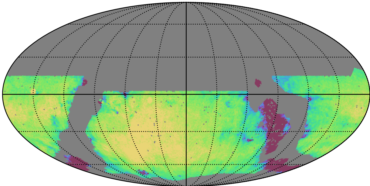
roll_pause_mjdp270_v3.4_10yrs WFD g band: Exgal_CoaddM5
