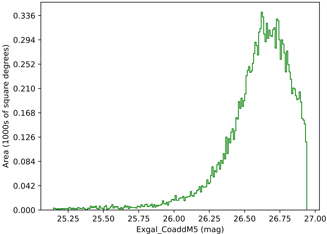
roll_pause_mjdp270_v3.4_10yrs WFD g band: Exgal_CoaddM5
