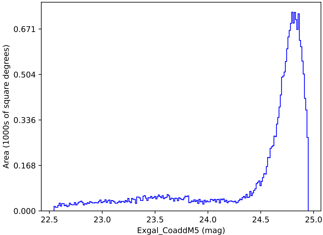
roll_pause_mjdp270_v3.4_10yrs All sky y band: Exgal_CoaddM5
