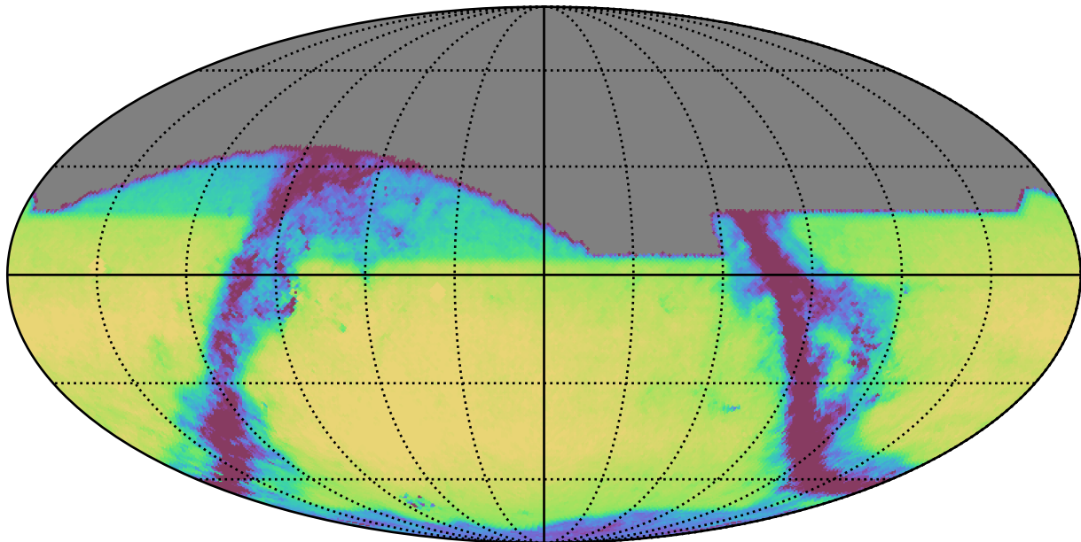
roll_pause_mjdp270_v3.4_10yrs All sky i band: Exgal_CoaddM5
