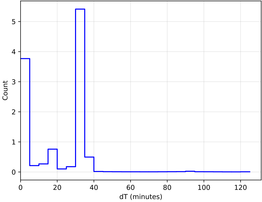
roll_pause_mjdp270_v3.4_10yrs WFD: DeltaT Histogram
